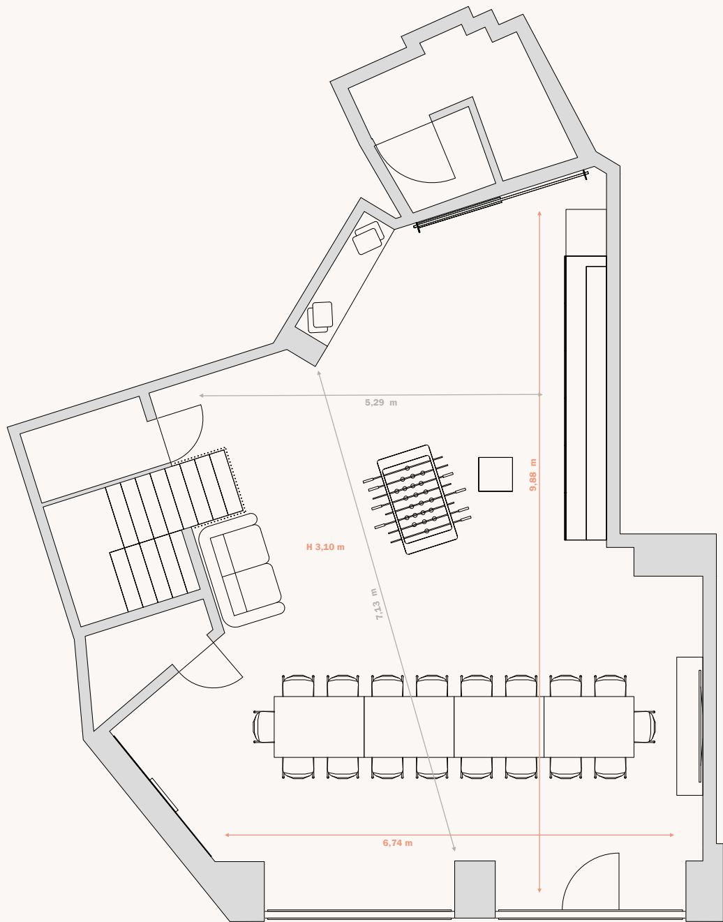
GROUND FLOOR
